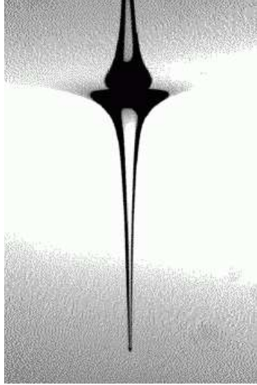
Figure 25.2: Water vortex in a rotating container. The upper part is the reflection of the vortex in the water surface. The radius of the drain-hole is a = 1 mm, the radius of the container is A = 20 cm, the asymptotic water level is L = 11 cm, and the whole apparatus rotates at \Omega = 18 rpm. After about 30 minutes the vortex stabilizes with a central dip of L - h_0 = 6 cm, or h_0 = 5 cm. The volume discharge through the drain is measured to be Q = 3.16 \text{ cm}^3 \text{ s}^{-1} corresponding to an average drain velocity of W = 101 \text{ cm s}^{-1} and a Reynolds number \text{Re}_z = 2328 . The circulation constant is C = 16.0 \text{ cm}^2 \text{ s}^{-1} , and the Rossby radius R = 2.9 cm. The core rotates more 50 times per second!
