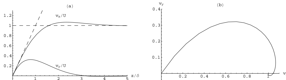
Figure 25.1: Plot of Ekman layer velocity components. (a) The velocity components as a function of height z . (b) Parametric plot of the velocities as a function of z leads to the characteristic Ekman spiral.
