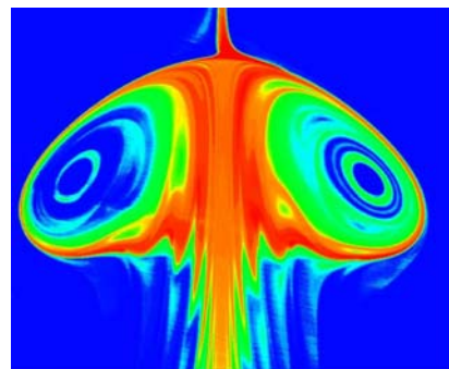
Figure 2: The vortex breakdown flow: Poincaré map extracted from experimental observations of the flow. [DRW and F. Sotiropoulos]
