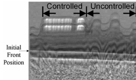
Figure 4: Formation of “fingers” in spreading of a film on a solid substrate (right side of figure) leads to a nonuniform coating. Small optically-induced surface-tension gradients (left side) suppress this instability.
