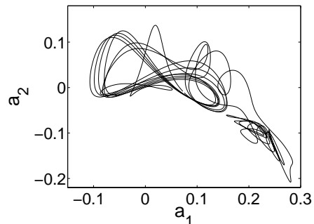
Figure 6: An unstable periodic solution of long period (roughly 30 \times the shortest periodic solution) embedded in 1-d Kuramoto-Sivashinsky turbulence. \{a_1, a_2\} Fourier modes projection from a 16-dimensional representation.
