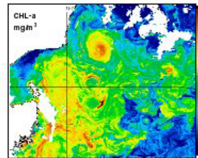
Figure 1: The SeaWiFS satellite observation of chlorophyll-a concentration.
