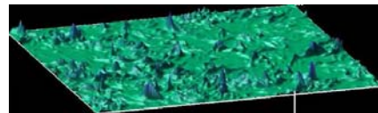
Figure 5: Instantaneous energy dissipation in a high resolution full 3-dimensional Navier-Stokes simulation.
