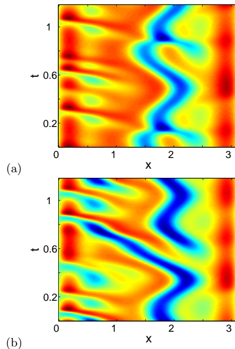
FIG. 5: Level plot of the space-time evolution u(x,t) for the two spatiotemporally periodic solutions of Fig. 4: (a) the evolution of p_1 , with start of a repeat after the cycle period T_1 = 0.744892 , and (b) one full period T_2 = 1.184668 in the evolution of p_2 .
