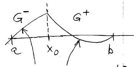
Solutions of homogeneous BVP
