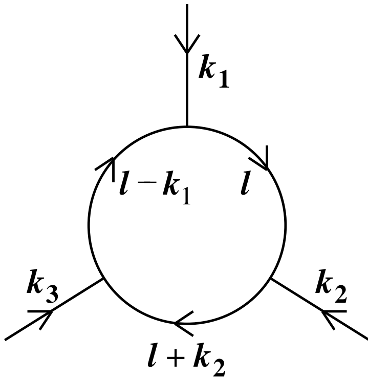
Figure 24: The O(g^3) correction to the vertex iV_3(k_1, k_2, k_3) .
