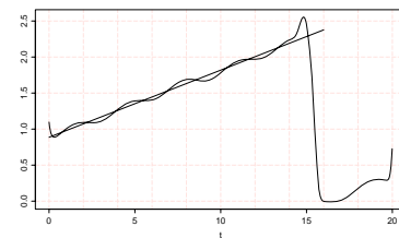
Fig. 15.4 A numerical estimate of the leading Lyapunov exponent for the Rössler system (2.15) from the dominant expanding eigenvalue formula (15.29). The leading Lyapunov exponent \lambda \approx 0.09 is positive, so numerics supports the hypothesis that the Rössler attractor is strange. (J. Mathiesen)
