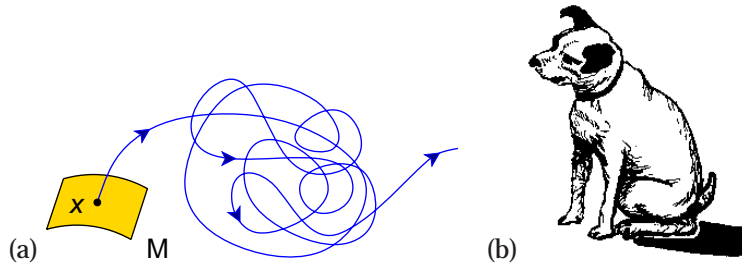
Fig. 15.1 (a) A typical chaotic trajectory explores the phase space with the long time visitation frequency building up the natural measure \rho_0(x) . (b) time average evaluated along an atypical trajectory such as a periodic orbit fails to explore the entire accessible state space. (A. Johansen)
