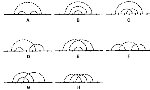
FIG. 2. Eight self-energy graphs of sixth order. There are two more graphs of this type obtained by inversion from graphs D and G . By inserting an external magnetic-field vertex in all possible ways in these ten diagrams, we can generate all fifty diagrams contributing to the sixth-order magnetic form factor.
