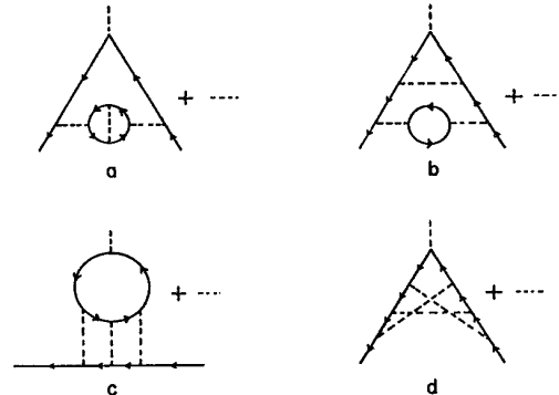
FIG. 1. (a) Typical diagram containing the fourth-order vacuum-polarization subgraph. There are three other diagrams of this type. (b) Typical diagram containing the second-order vacuum-polarization subgraph. There are altogether twelve diagrams of this type. (c) Typical diagram containing the photon-photon scattering subgraph. Six diagrams belong to this group. (d) Typical diagram that contains no vacuum-polarization subgraph. There are altogether fifty diagrams of this type.
