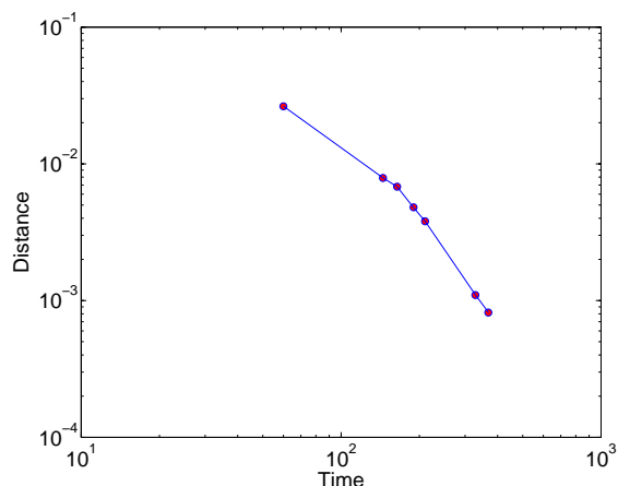
FIGURE 9. The axes correspond to the T and \delta columns in Table 4. The plot is for Re = 2500 . Each point corresponds to a certain stage in the sequence of optimizations used to find a disturbance of the laminar flow such that the disturbed flow evolves and hits the traveling wave.
